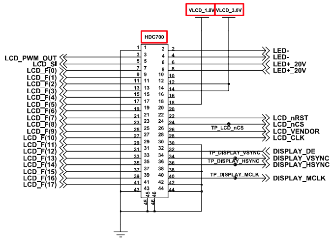
LCD CONN
